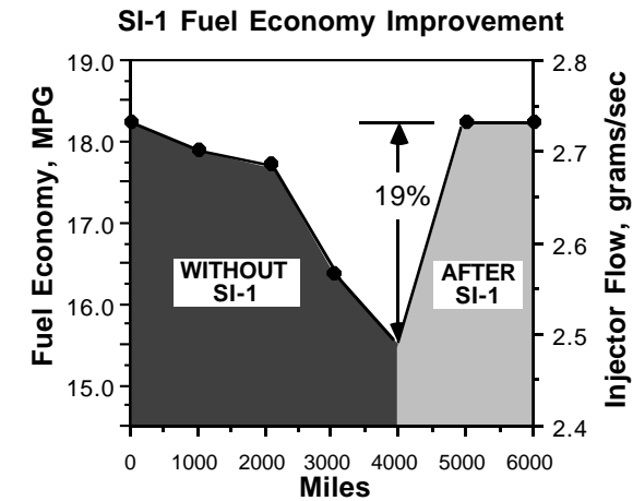
Figure 2: The deterioration of fuel economy and injector flow with subsequent restoration using one bottle of SI-1.
