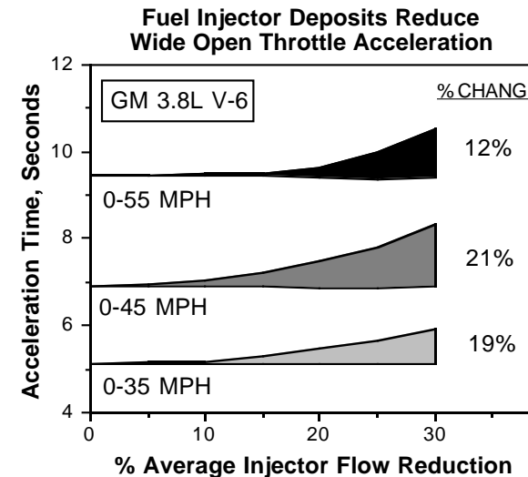
Figure 3: By reducing injector plugging, SI-1 can improve acceleration times as much as 20%.
